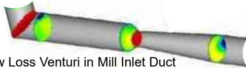
Low Loss Venturi in Mill Inlet Duct
